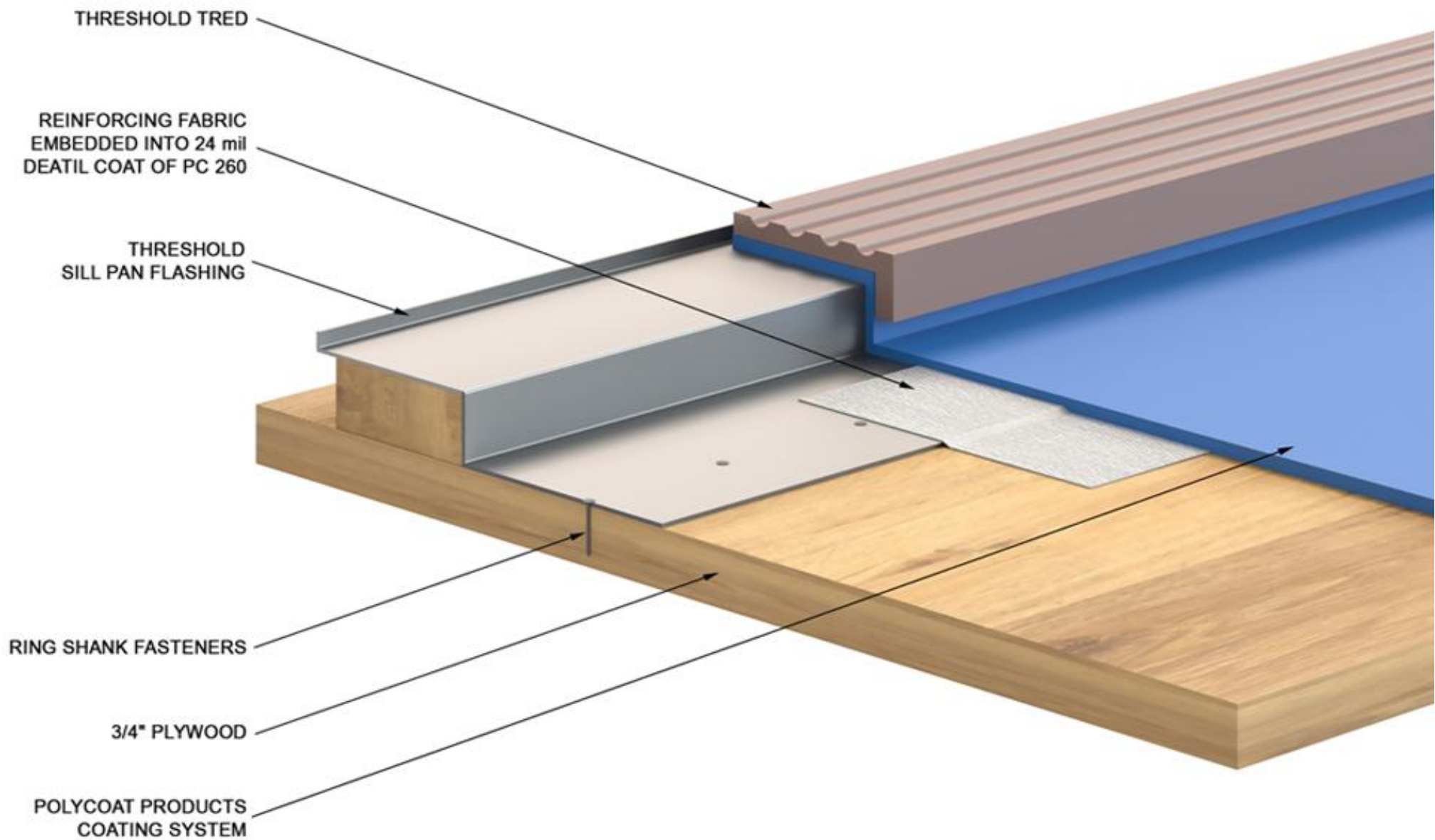
19- SLIDING DOOR THRESHOLD (Plywood Substance)
