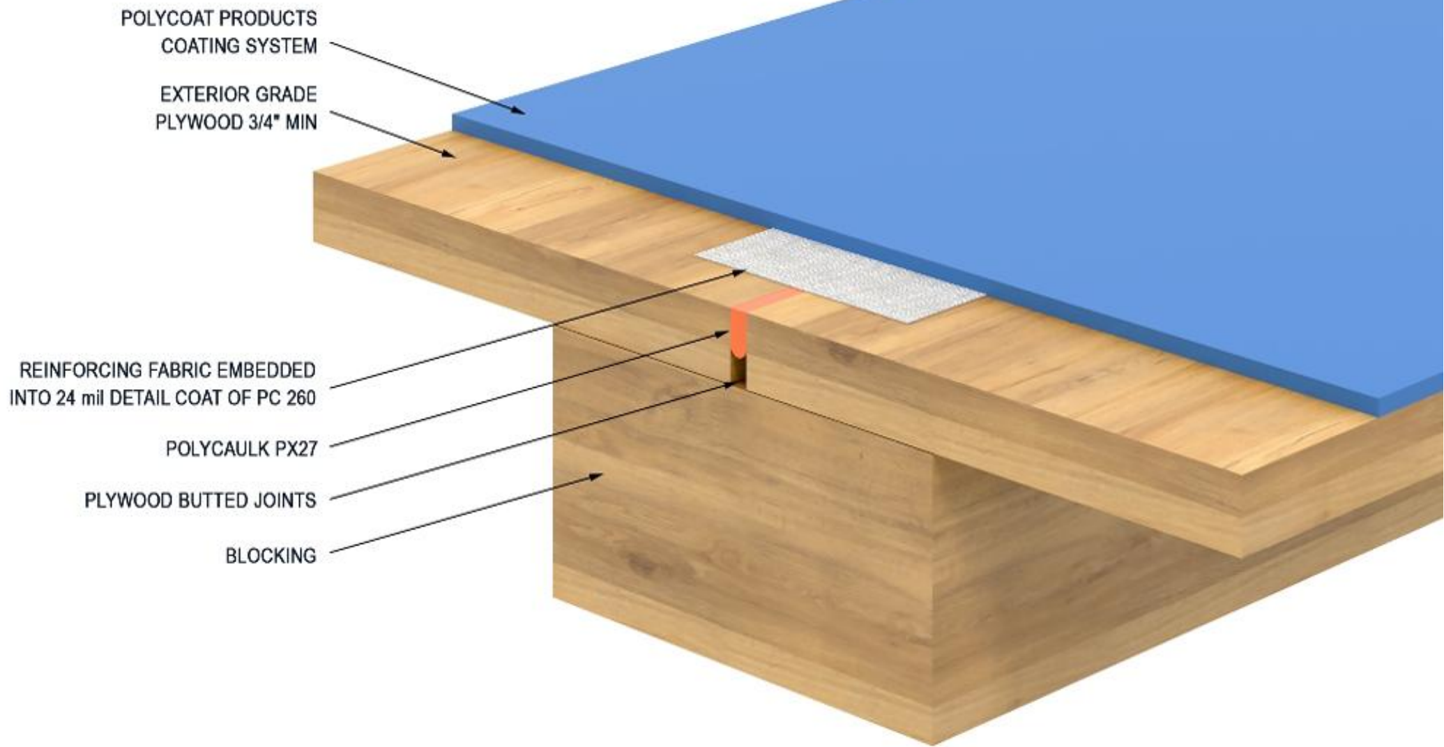
24- PLYWOOD JOINT
