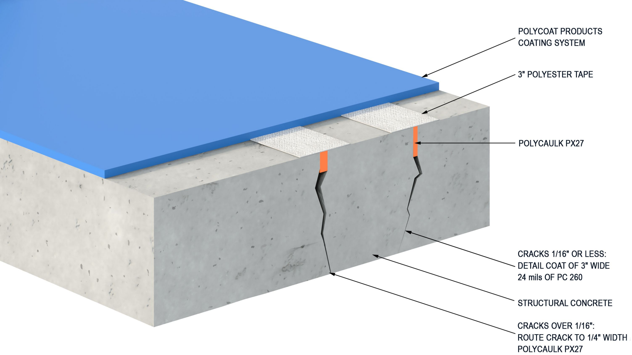
21- CRACK TREATMENT
